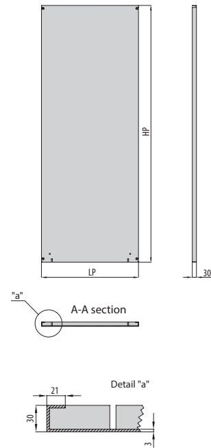
Mounting plate
