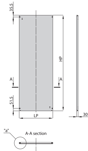
Mounting plate
