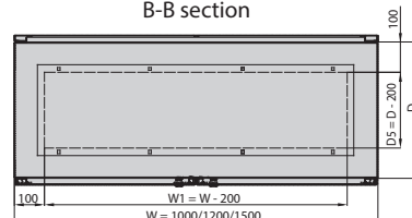
B-B section
