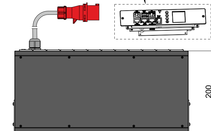
VIEW B
