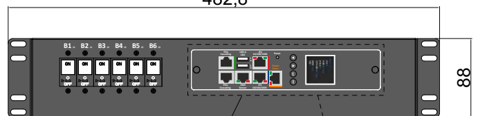
VIEW B
