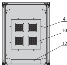
A-A section (800 mm deep cabinet)
