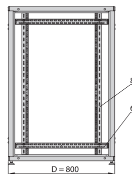
Side view (800 mm deep cabinet)
