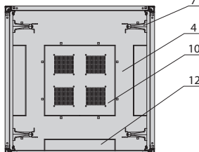
C-C section (800 mm deep cabinet)
