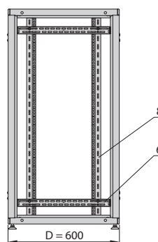
Side view (600 mm deep cabinet)
